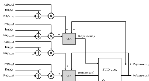
Fig. 2. Auto-correlator for the coarse time synchronization
